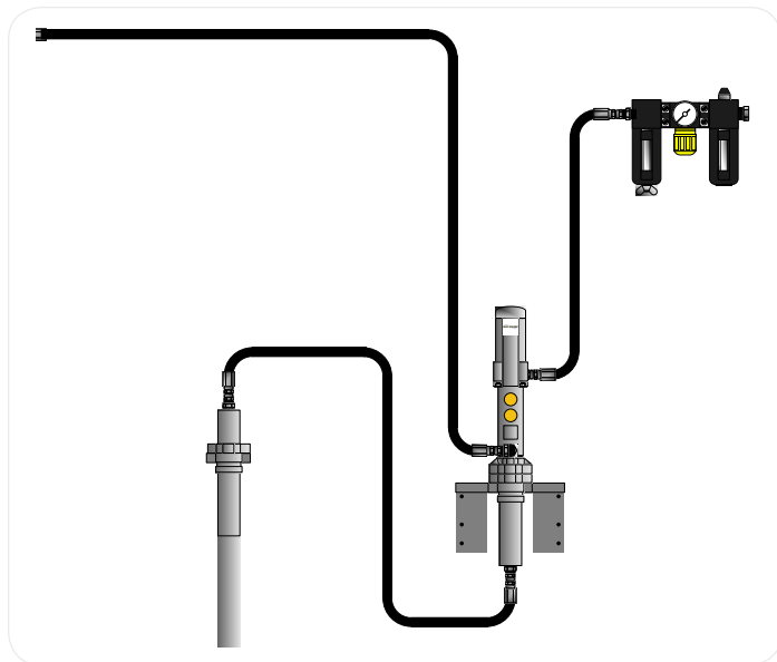
Typical wall mount hook-up.
