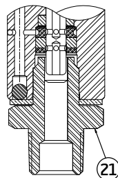
SINGLE MOUNTED FL44-DM INJECTOR (3/8" NPT)
