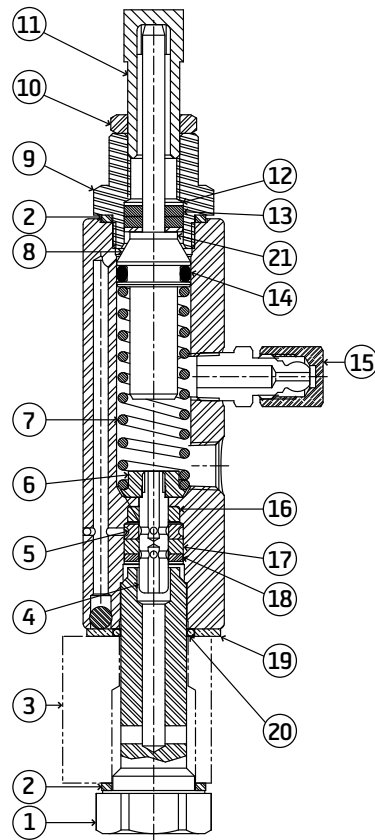
MANIFOLD MOUNTED FL44 INJECTOR
